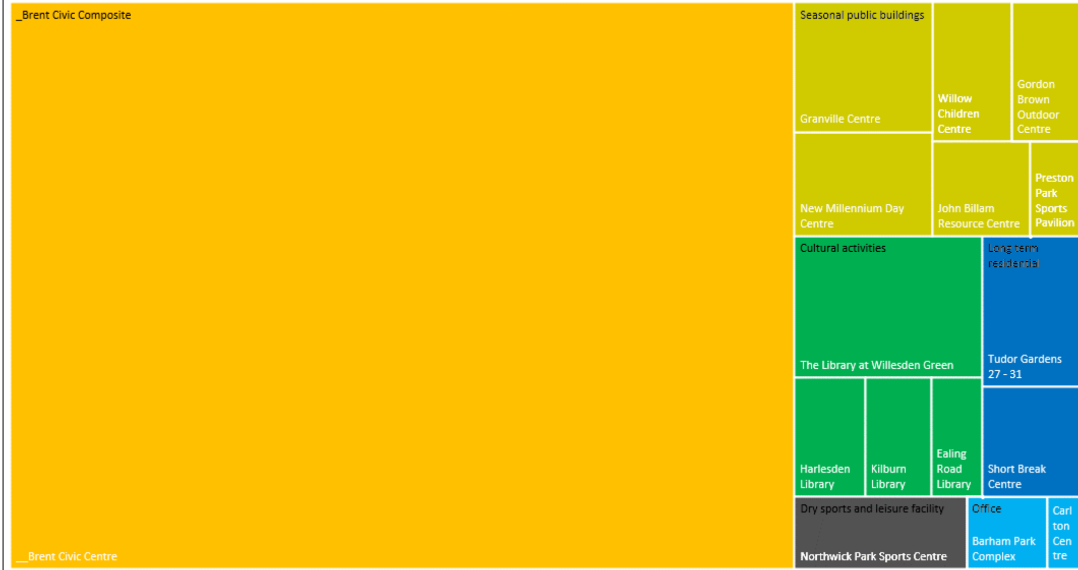
Figure 1: Tree Map of 2020-21 carbon emissions from the project site
